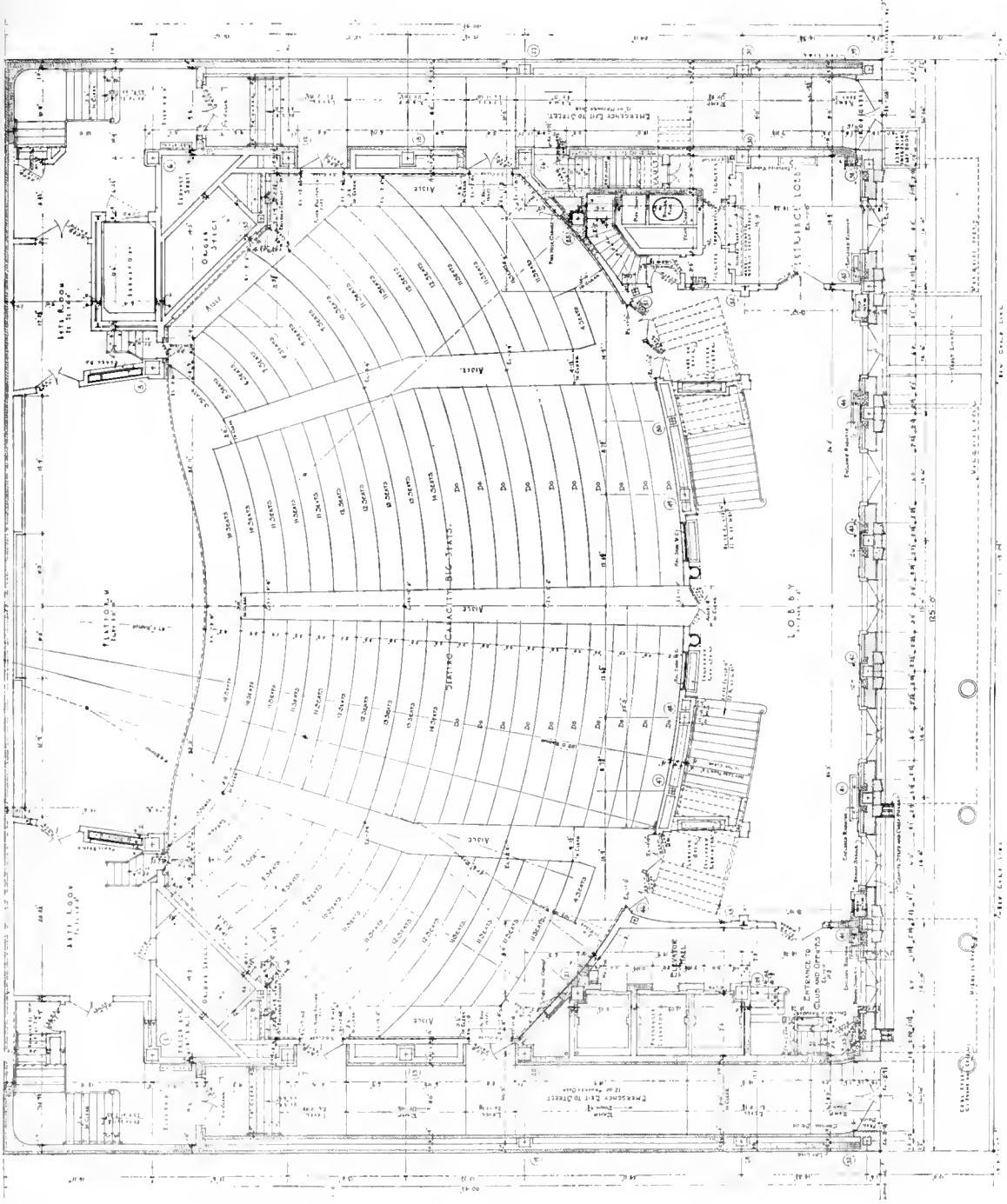
FIRST FLOOR PLAN THE TOWN HALL, NEW YORK CITY McKIM, MEAD & WHITE, ARCHITECTS
